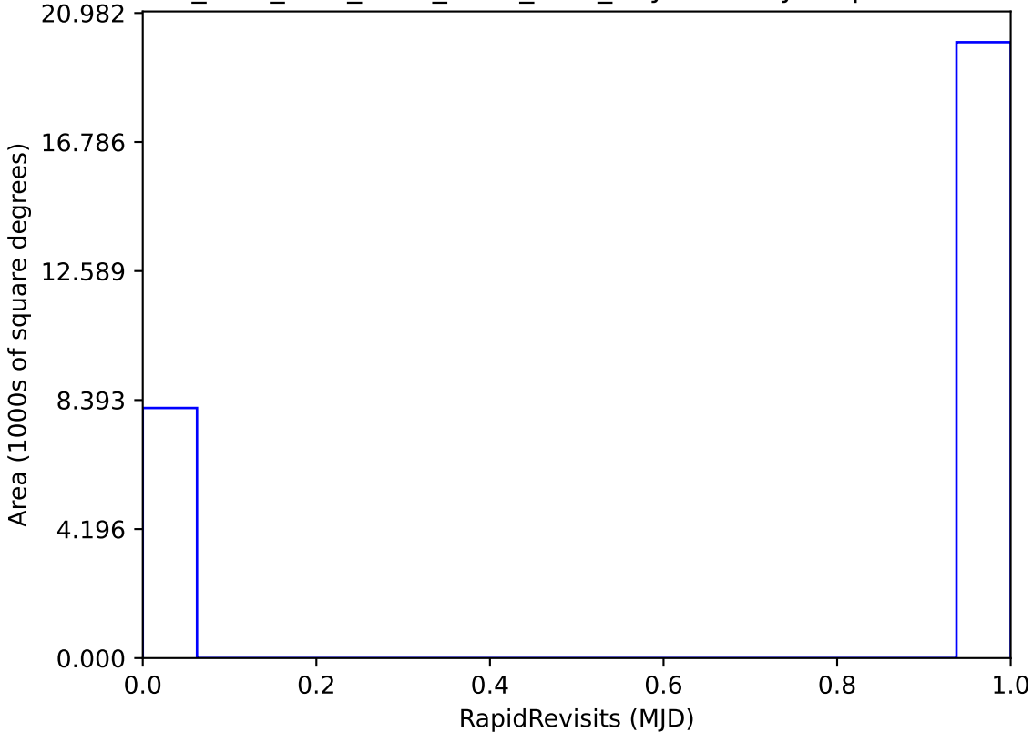
ddf_acor_sf30_lsf40_lsr20_v3.4_10yrs All sky: RapidRevisits
