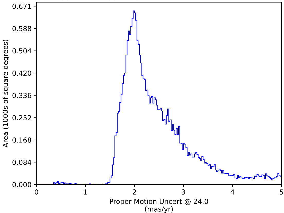
ddf_acor_sf30_lsf40_lsr20_v3.4_10yrs All sky: Proper Motion Uncert @ 24.0
