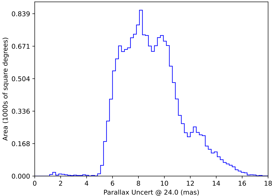
ddf_acor_sf30_lsf40_lsr20_v3.4_10yrs WFD: Parallax Uncert @ 24.0
