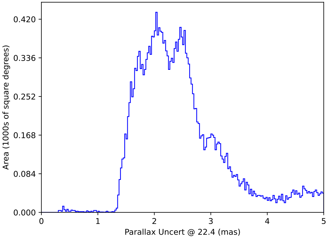
ddf_acor_sf30_lsf40_lsr20_v3.4_10yrs All sky: Parallax Uncert @ 22.4
