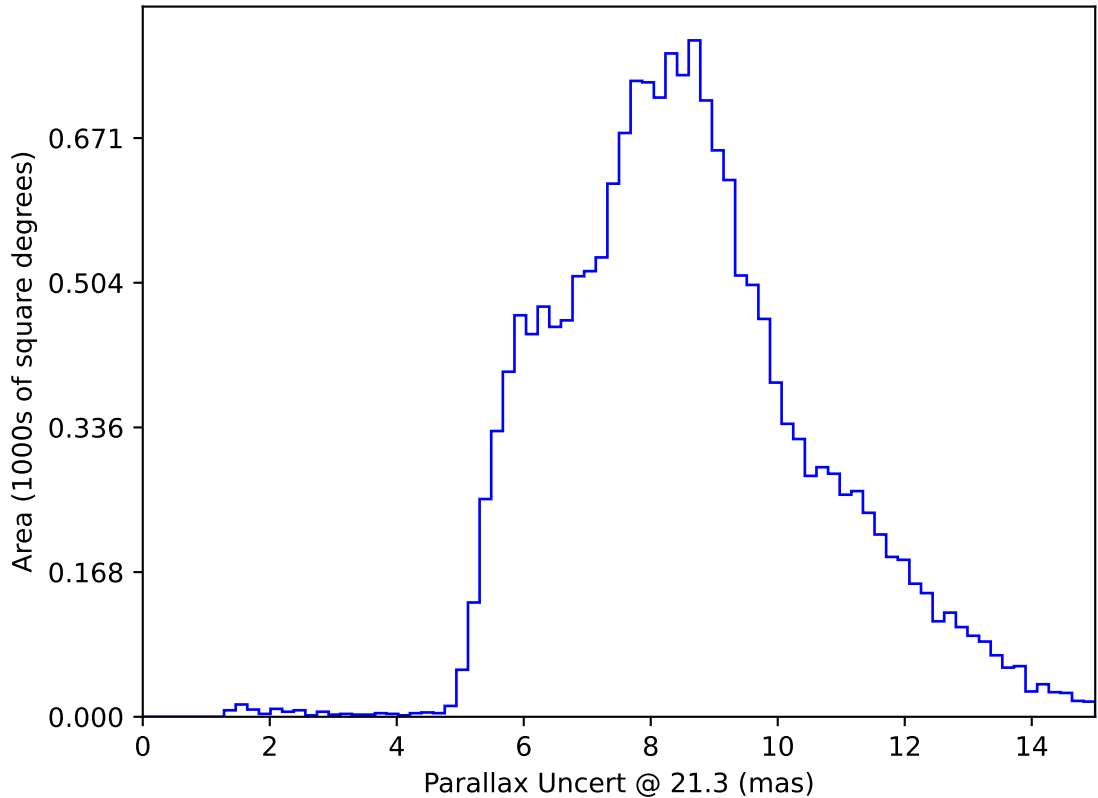
ddf_acor_sf30_lsf40_lsr20_v3.4_10yrs WFD y band only: Parallax Uncert @ 21.3
