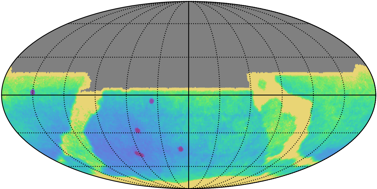
ddf_acor_sf30_lsf40_lsr20_v3.4_10yrs All sky y band only: Parallax Uncert @ 21.3
