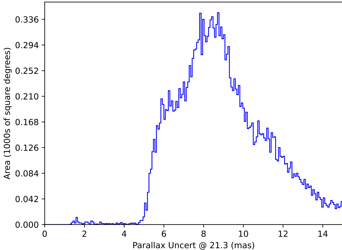
ddf_acor_sf30_lsf40_lsr20_v3.4_10yrs All sky y band only: Parallax Uncert @ 21.3
