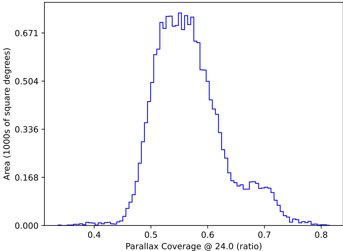
ddf_acor_sf30_lsf40_lsr20_v3.4_10yrs WFD: Parallax Coverage @ 24.0
