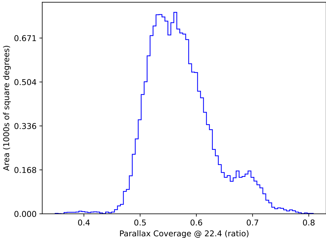
ddf_acor_sf30_lsf40_lsr20_v3.4_10yrs WFD: Parallax Coverage @ 22.4
