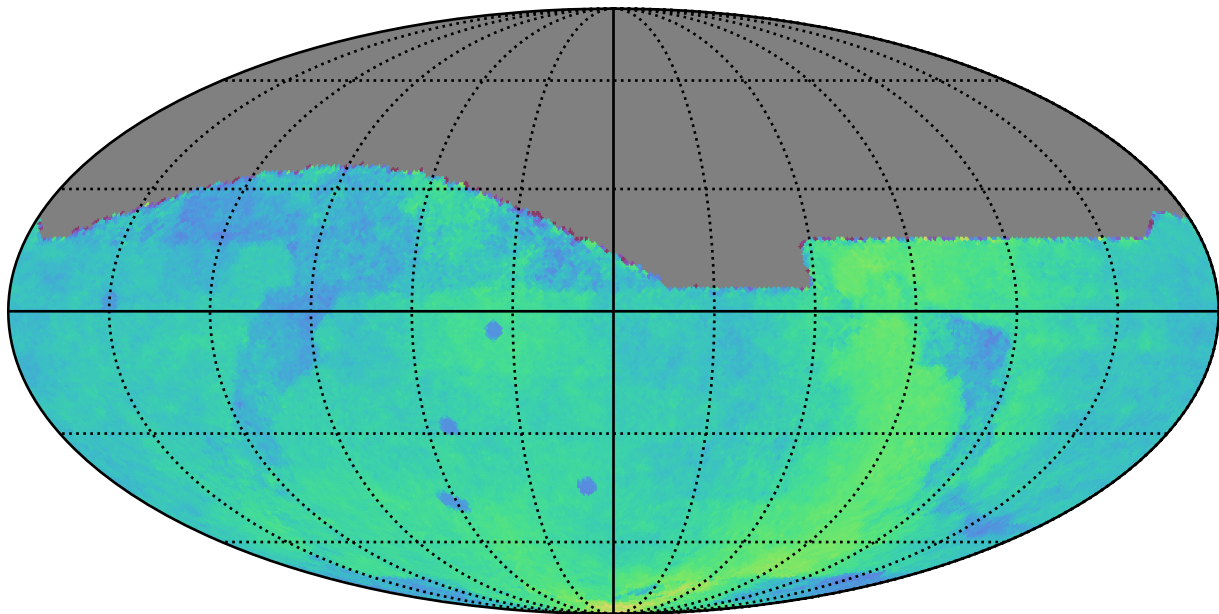
ddf_acor_sf30_lsf40_lsr20_v3.4_10yrs All sky: Parallax Coverage @ 22.4
