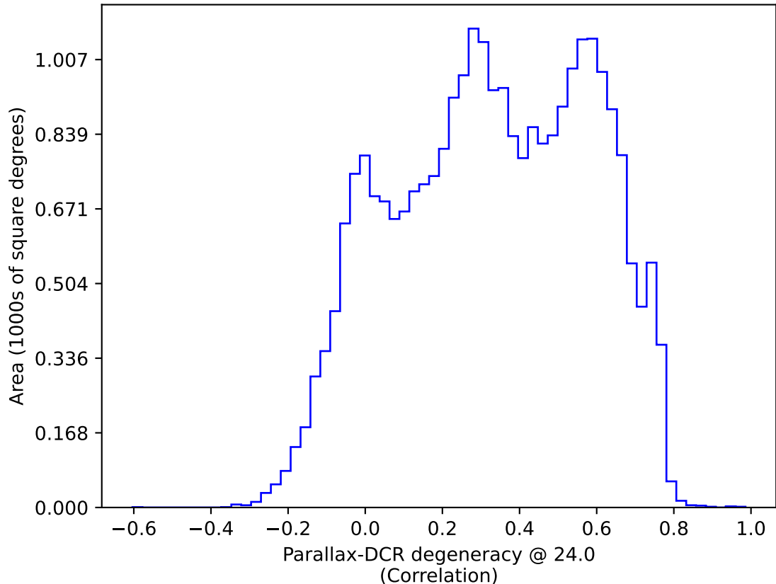
ddf_acor_sf30_lsf40_lsr20_v3.4_10yrs All sky: Parallax-DCR degeneracy @ 24.0
