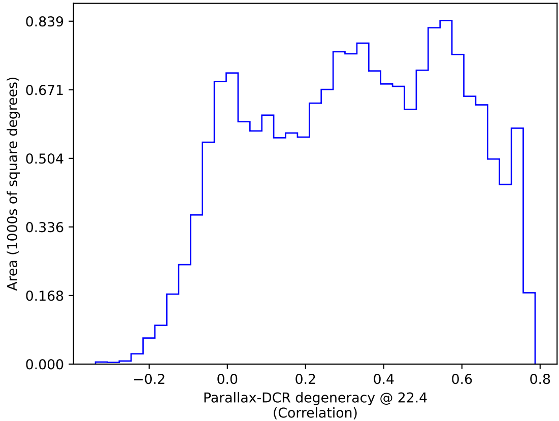
ddf_acor_sf30_lsf40_lsr20_v3.4_10yrs WFD: Parallax-DCR degeneracy @ 22.4
