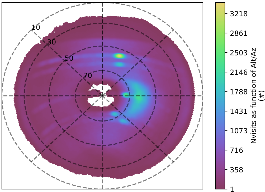
ddf_acor_sf30_lsf40_lsr20_v3.4_10yrs z band: Nvisits as function of Alt/Az
