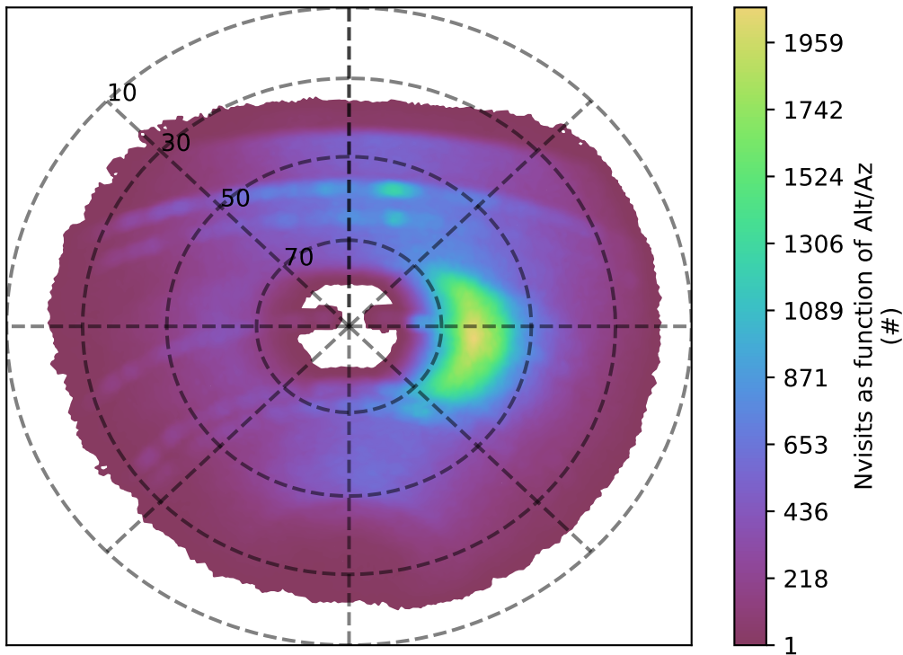
ddf_acor_sf30_lsf40_lsr20_v3.4_10yrs y band: Nvisits as function of Alt/Az
