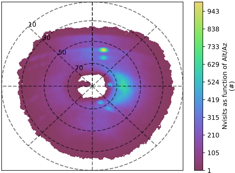
ddf_acor_sf30_lsf40_lsr20_v3.4_10yrs u band: Nvisits as function of Alt/Az
