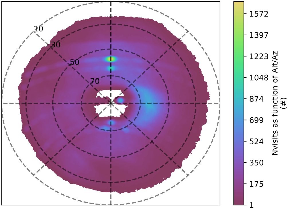
ddf_acor_sf30_lsf40_lsr20_v3.4_10yrs g band: Nvisits as function of Alt/Az
