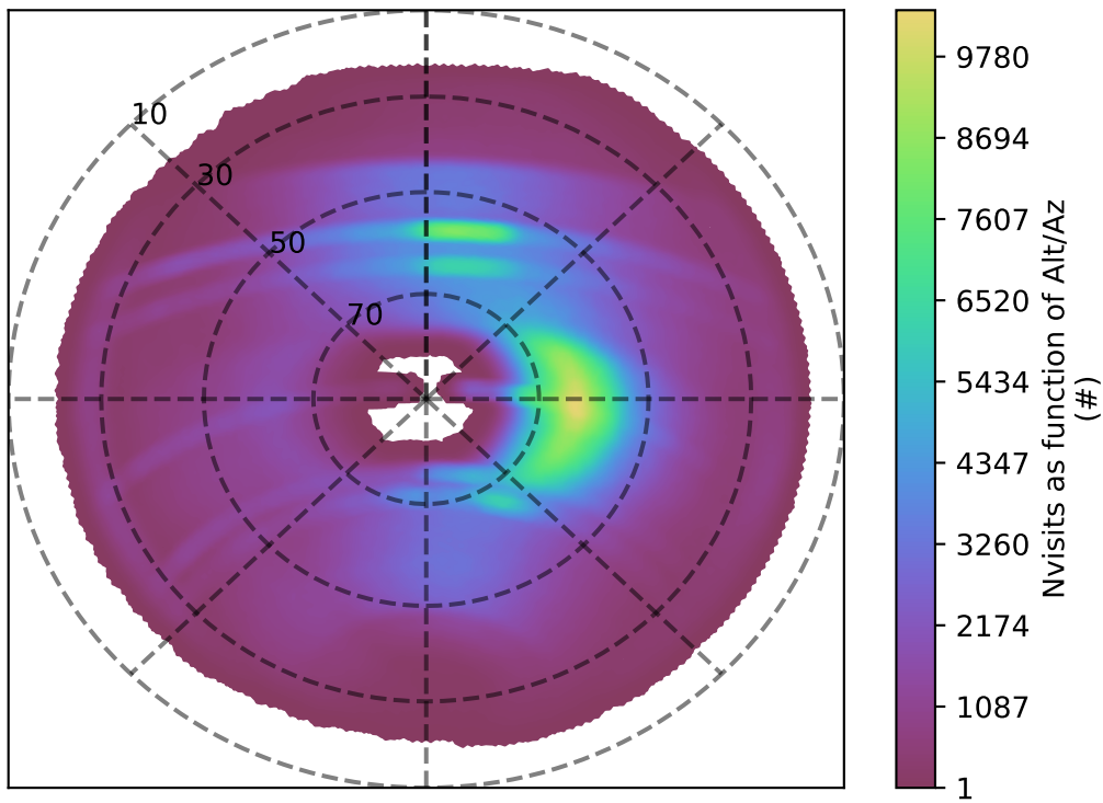
ddf_acor_sf30_lsf40_lsr20_v3.4_10yrs all bands: Nvisits as function of Alt/Az
