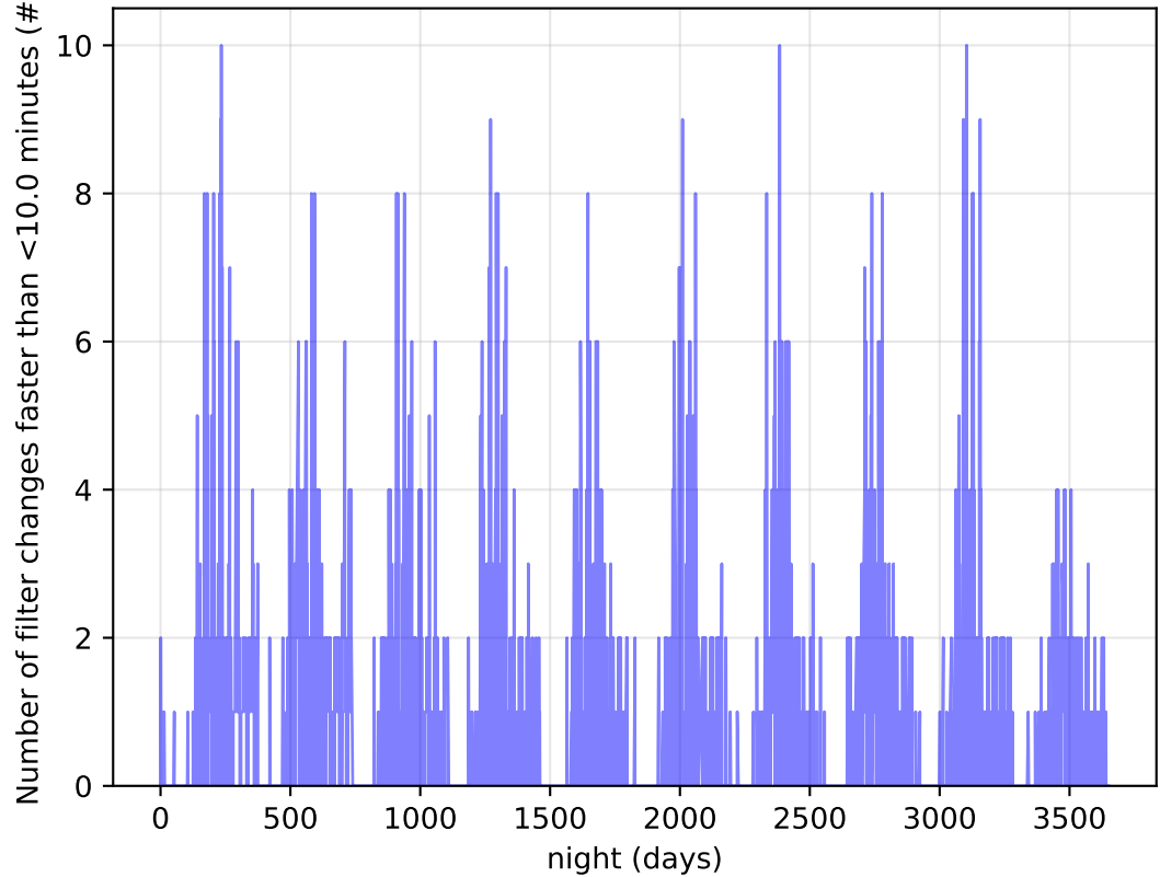
ddf_acor_sf30_Isf40_Isr20_v3.4_10yrs Per Night: Number of filter changes faster than <10.0 minutes
