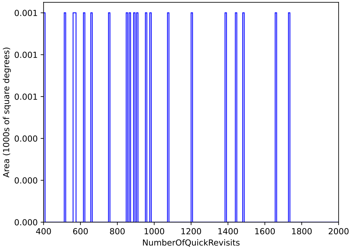
ddf_acor_sf30_ls40_lsr20_v3.4_10yrs All sky: NumberOfQuickRevisits
