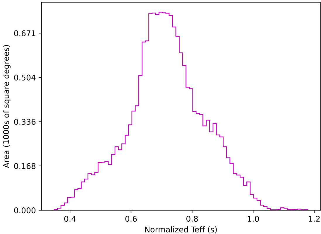
ddf_acor_sf30_lsf40_lsr20_v3.4_10yrs WFD z band: Normalized Teff
