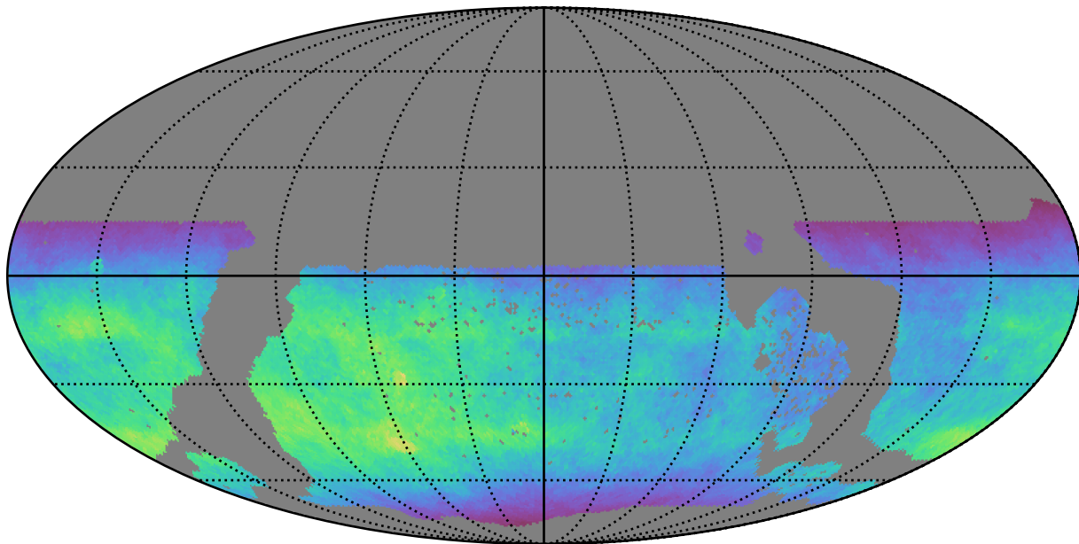
ddf_acor_sf30_lsf40_lsr20_v3.4_10yrs WFD y band: Normalized Teff
