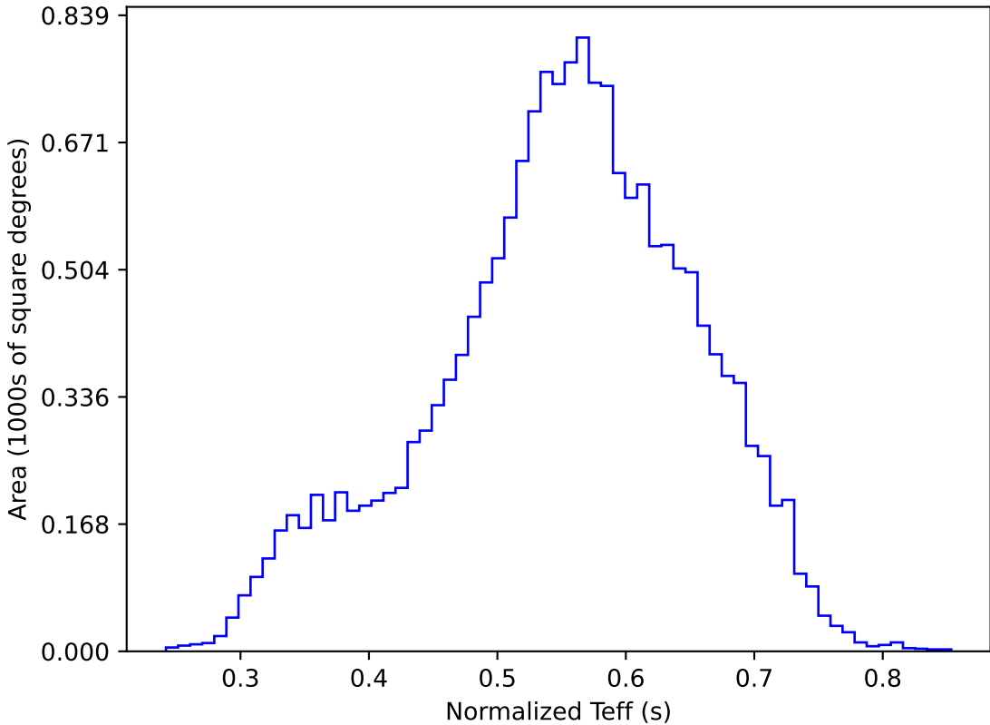
ddf_acor_sf30_lsf40_lsr20_v3.4_10yrs WFD y band: Normalized Teff
