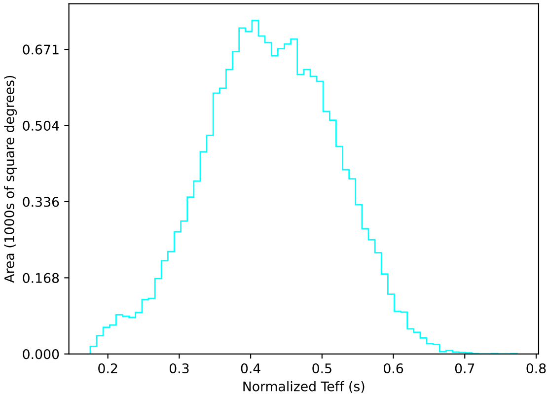
ddf_acor_sf30_lsf40_lsr20_v3.4_10yrs WFD u band: Normalized Teff
