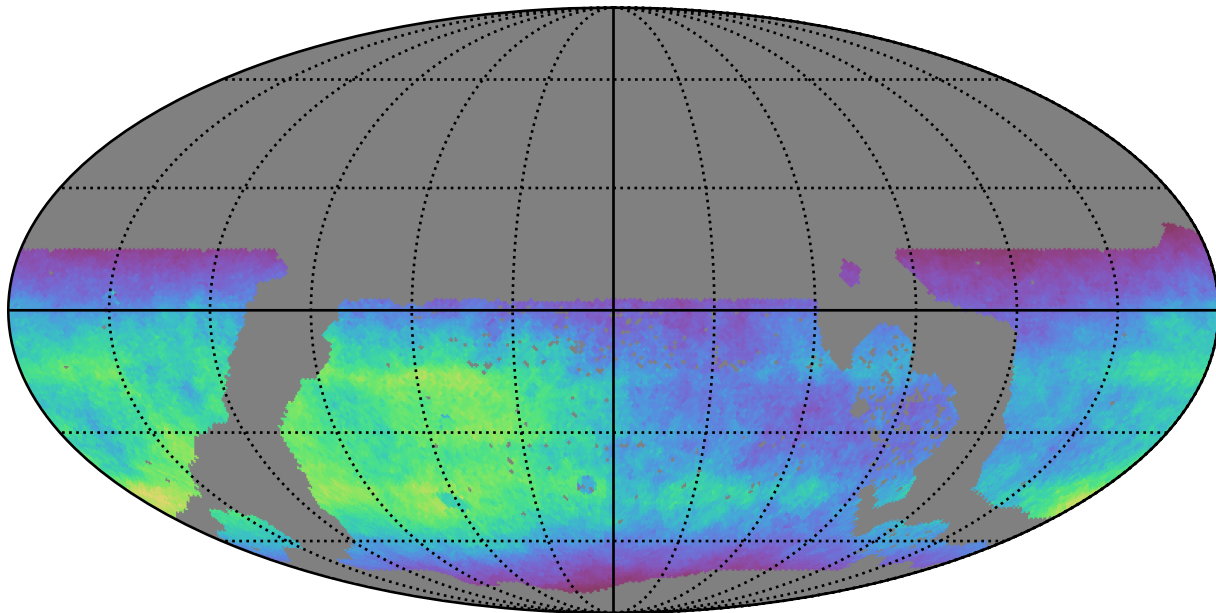
ddf_acor_sf30_lsf40_lsr20_v3.4_10yrs WFD r band: Normalized Teff
