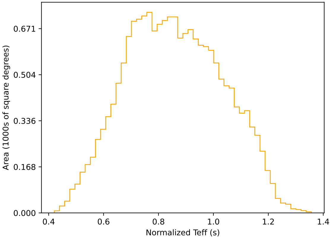
ddf_acor_sf30_lsf40_lsr20_v3.4_10yrs WFD r band: Normalized Teff
