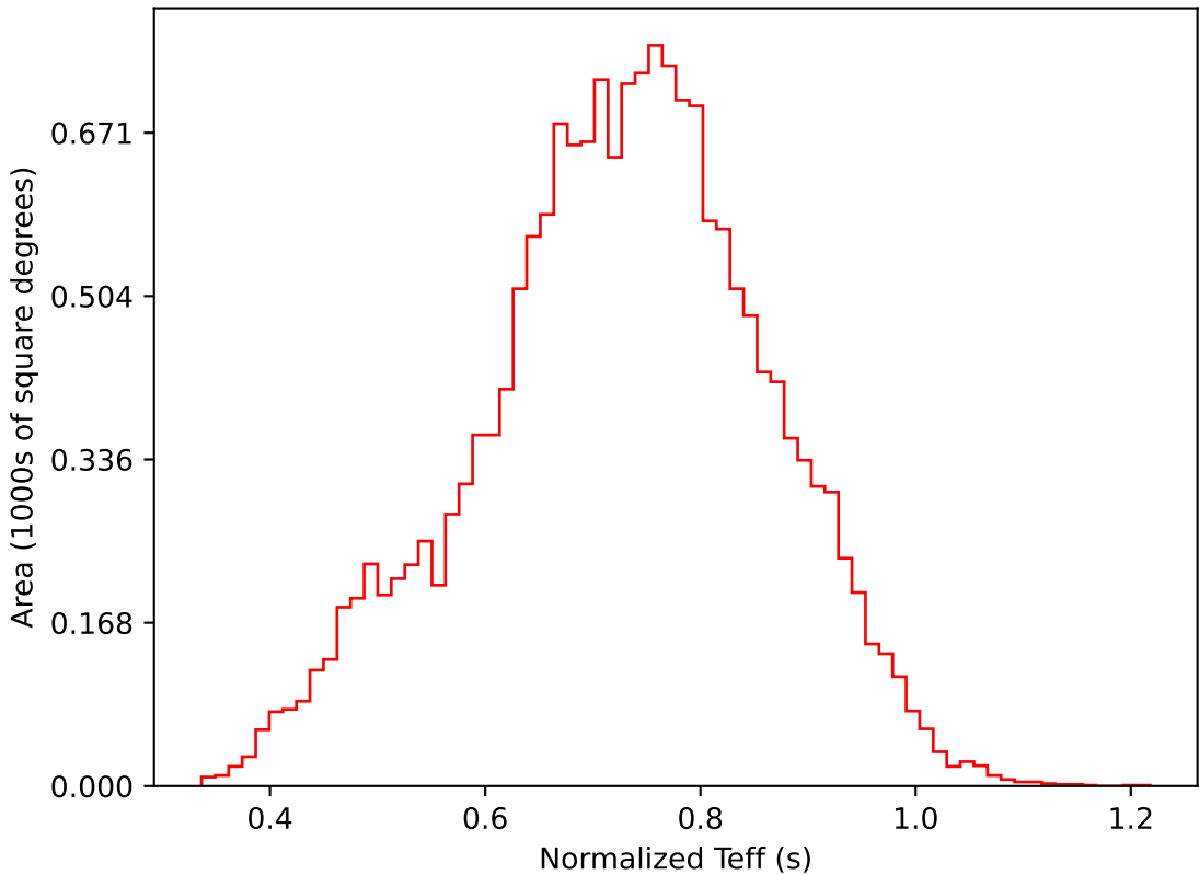
ddf_acor_sf30_lsf40_lsr20_v3.4_10yrs WFD i band: Normalized Teff
