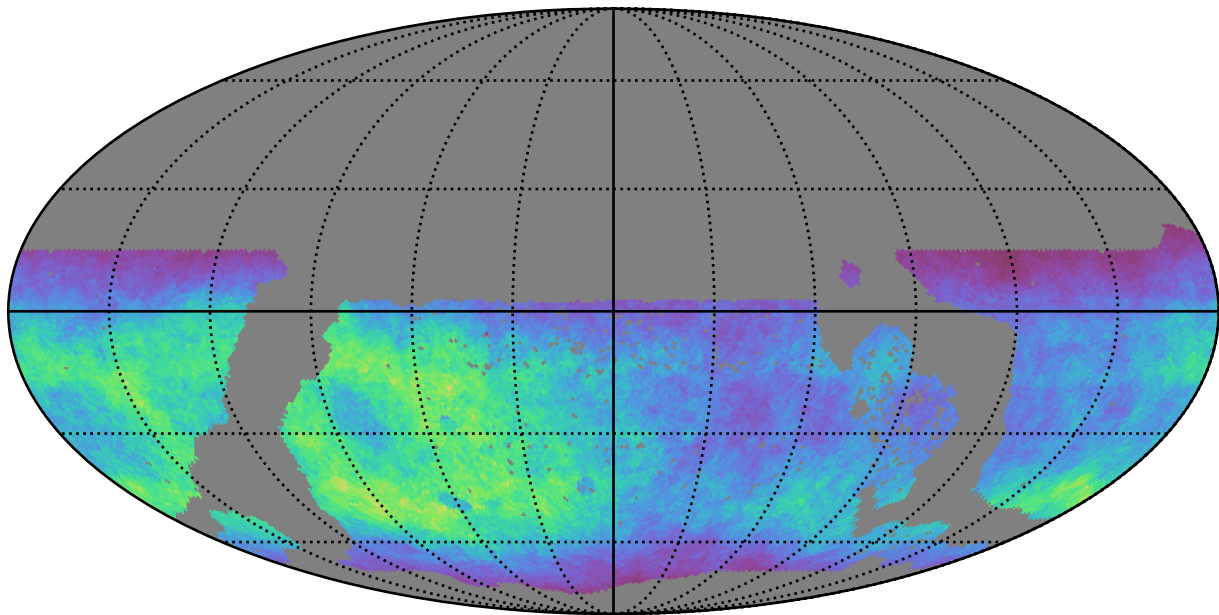
ddf_acor_sf30_lsf40_lsr20_v3.4_10yrs WFD g band: Normalized Teff
