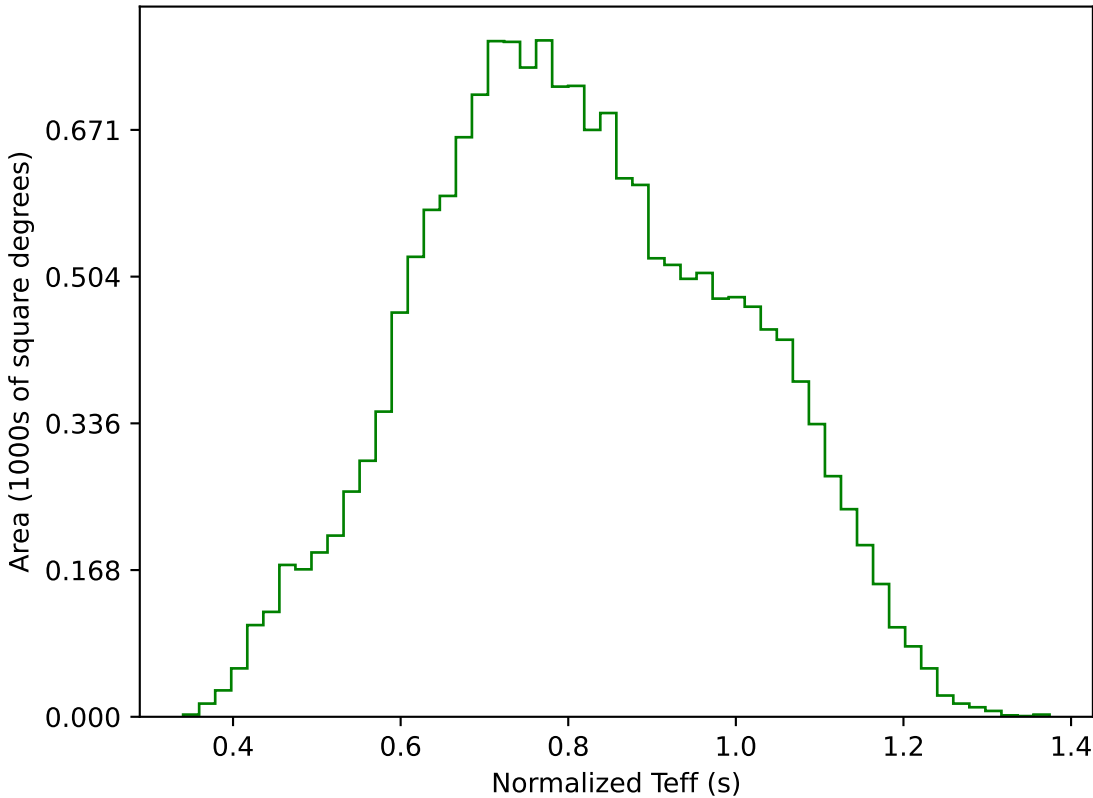
ddf_acor_sf30_lsf40_lsr20_v3.4_10yrs WFD g band: Normalized Teff
