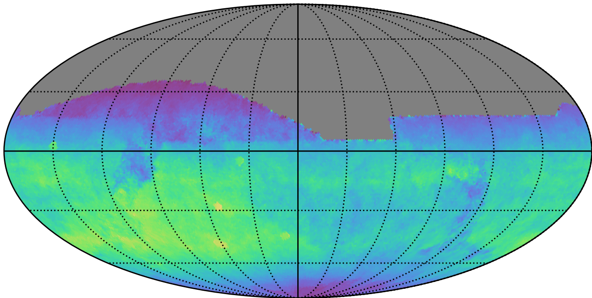
ddf_acor_sf30_lsf40_lsr20_v3.4_10yrs All sky z band: Normalized Teff
