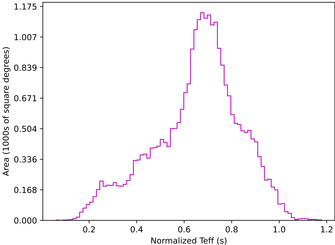
ddf_acor_sf30_lsf40_lsr20_v3.4_10yrs All sky z band: Normalized Teff
