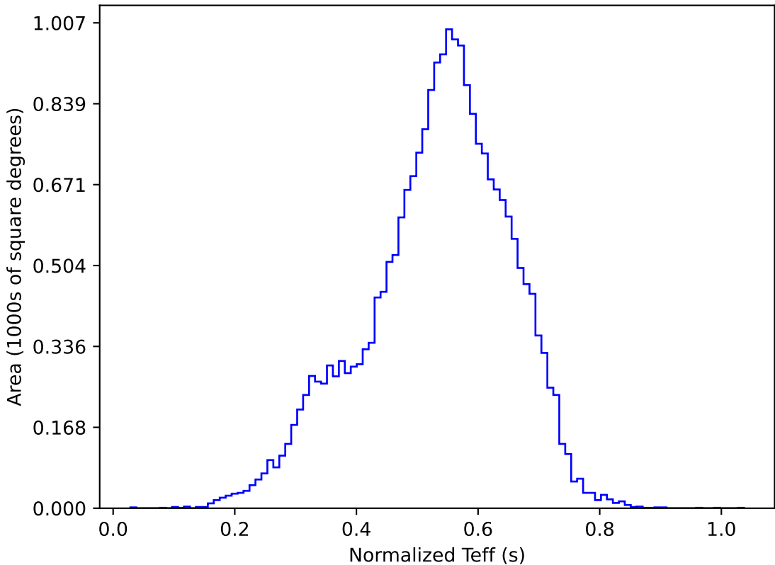
ddf_acor_sf30_lsf40_lsr20_v3.4_10yrs All sky y band: Normalized Teff
