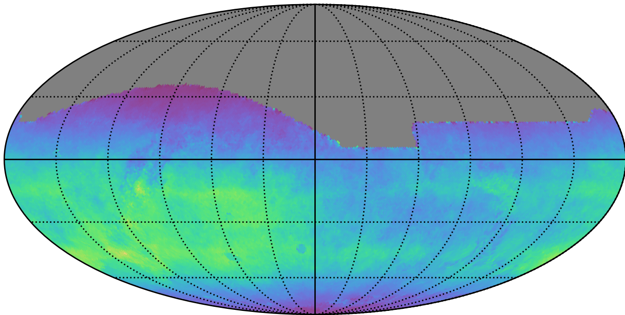
ddf_acor_sf30_lsf40_lsr20_v3.4_10yrs All sky r band: Normalized Teff
