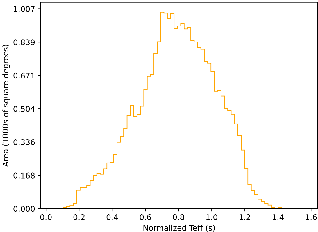
ddf_acor_sf30_lsf40_lsr20_v3.4_10yrs All sky r band: Normalized Teff
