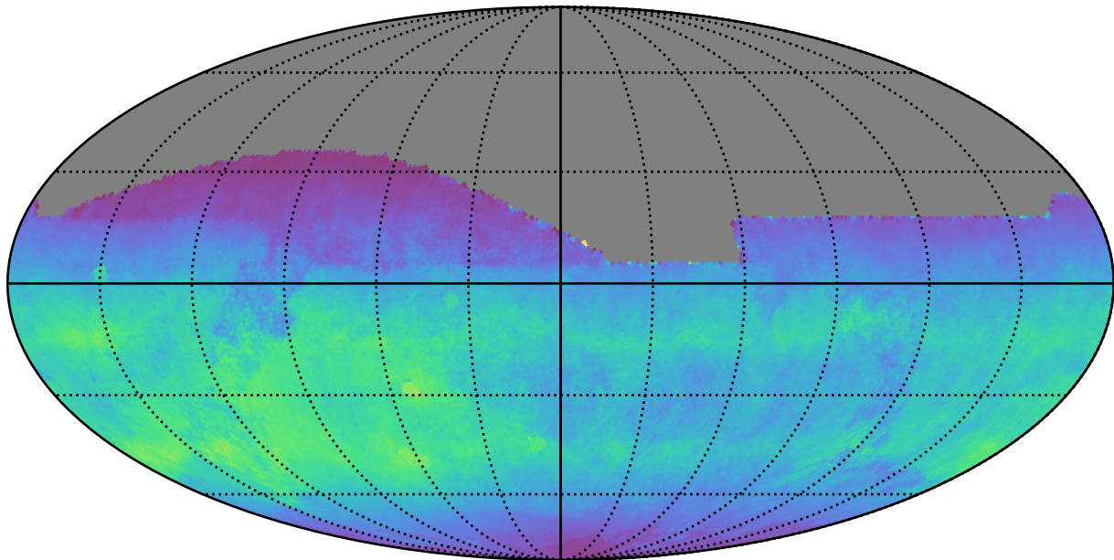
ddf_acor_sf30_lsf40_lsr20_v3.4_10yrs All sky i band: Normalized Teff
