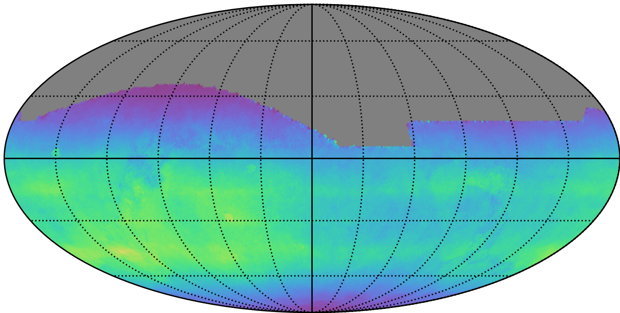
ddf_acor_sf30_lsf40_lsr20_v3.4_10yrs All sky all bands: Normalized Teff
