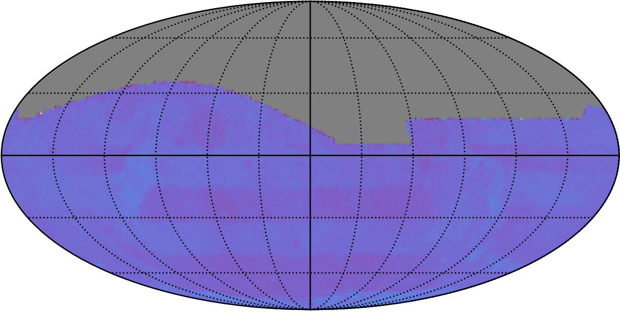
ddf_acor_sf30_lsf40_lsr20_v3.4_10yrs All sky: Normalized Proper Motion Uncert @ 24.0
