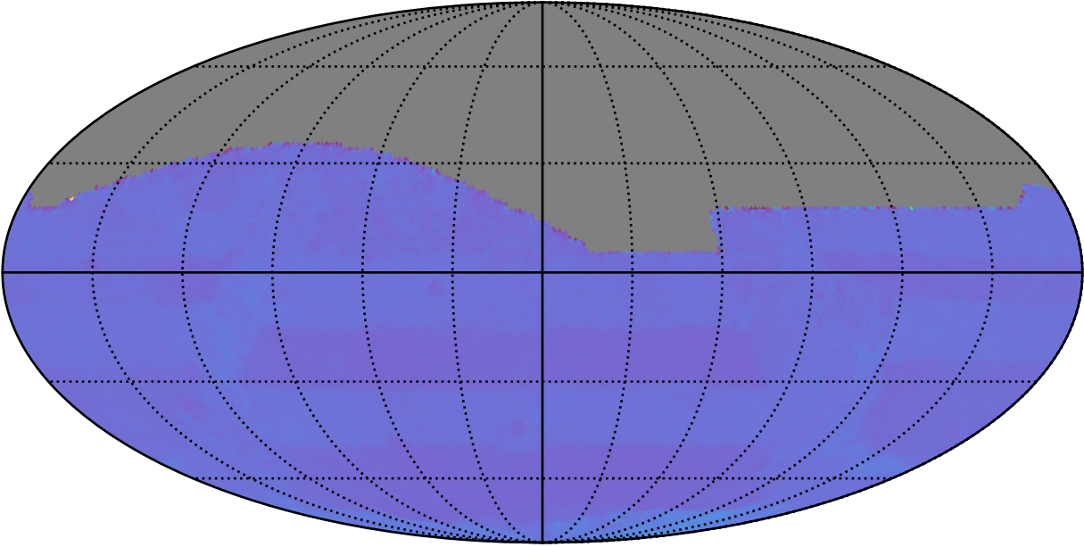
ddf_acor_sf30_lsf40_lsr20_v3.4_10yrs All sky: Normalized Proper Motion Uncert @ 20.5
