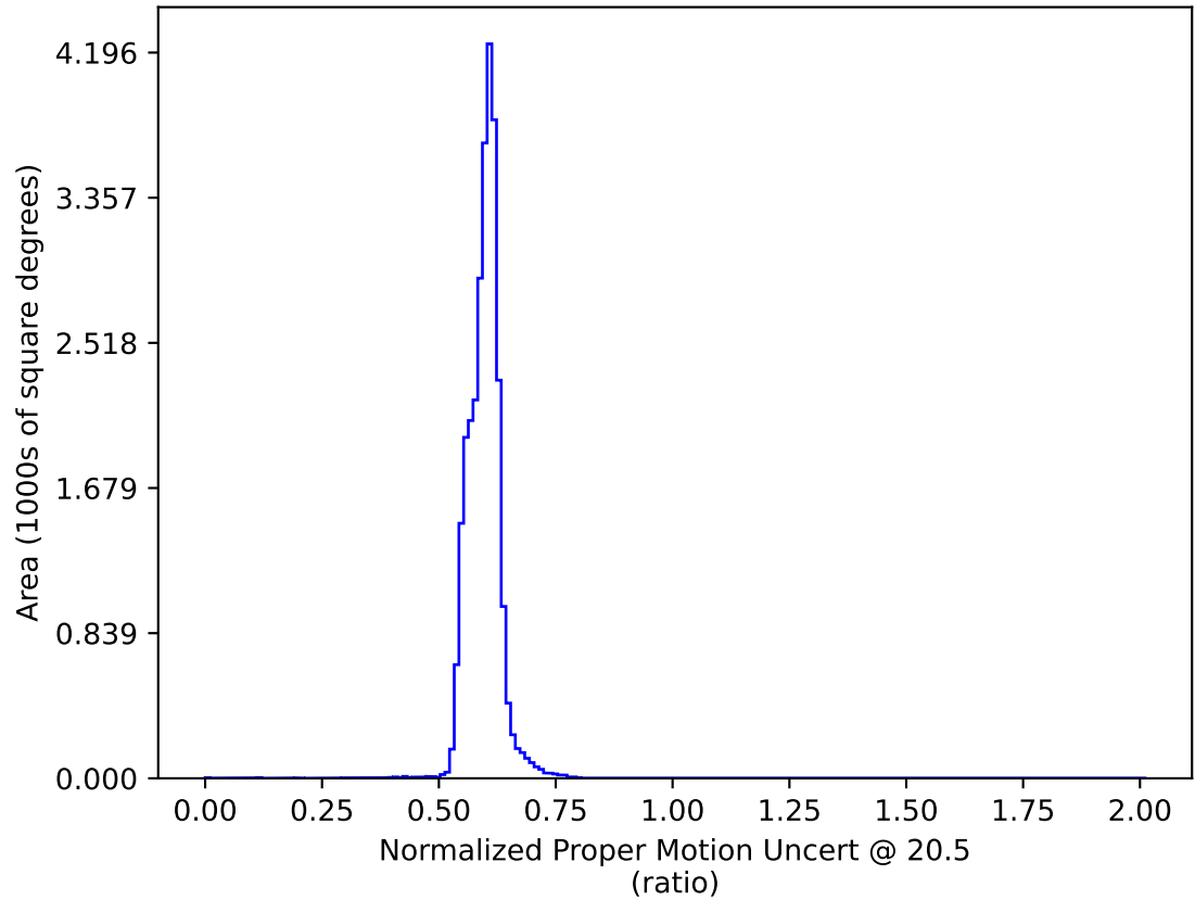
ddf_acor_sf30_lsf40_lsr20_v3.4_10yrs All sky: Normalized Proper Motion Uncert @ 20.5
