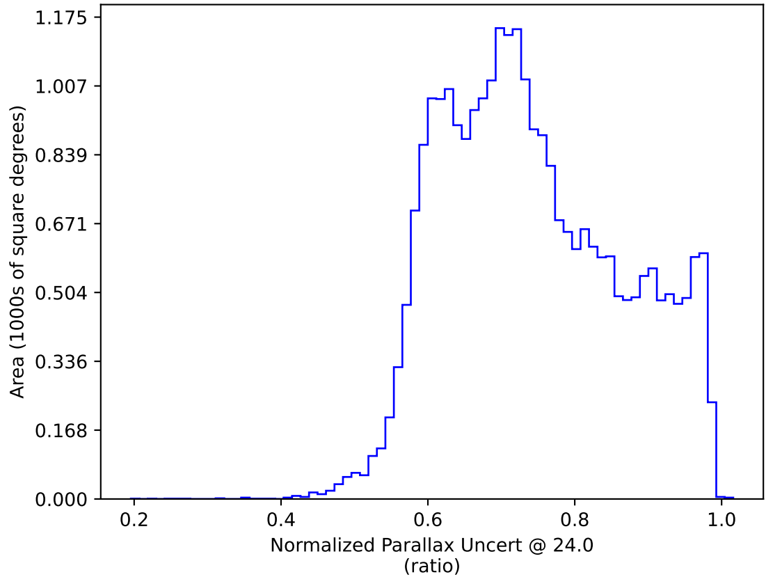
ddf_acor_sf30_lsf40_lsr20_v3.4_10yrs All sky: Normalized Parallax Uncert @ 24.0
