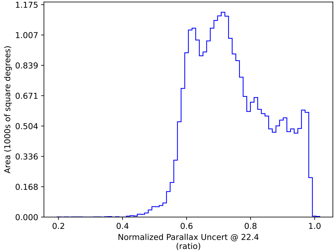
ddf_acor_sf30_lsf40_lsr20_v3.4_10yrs All sky: Normalized Parallax Uncert @ 22.4
