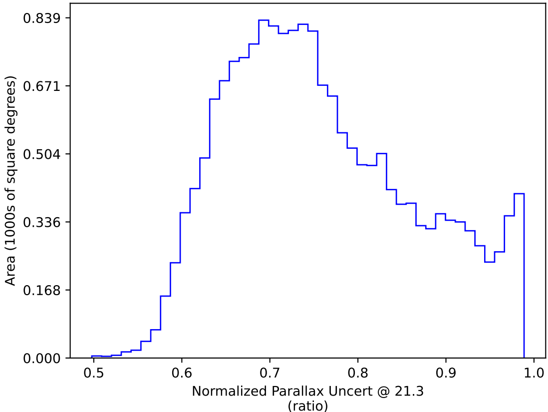
ddf_acor_sf30_lsf40_lsr20_v3.4_10yrs WFD y band only: Normalized Parallax Uncert @ 21.3
