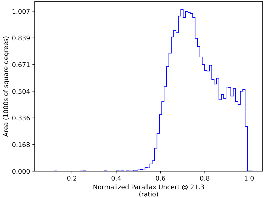
ddf_acor_sf30_lsf40_lsr20_v3.4_10yrs All sky y band only: Normalized Parallax Uncert @ 21.3
