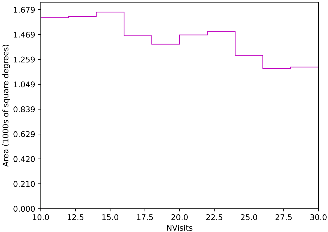
ddf_acor_sf30_lsf40_lsr20_v3.4_10yrs Yr 3-4 z band: NVisits
