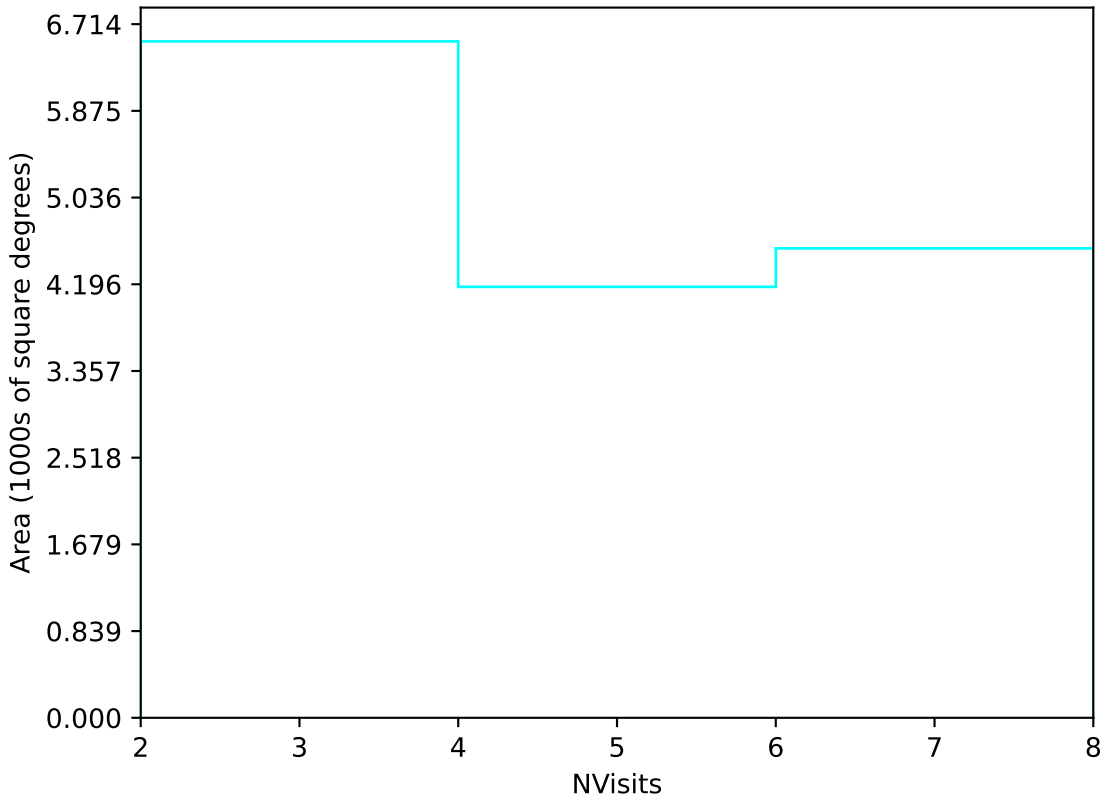
ddf_acor_sf30_lsf40_lsr20_v3.4_10yrs Yr 3-4 u band: NVisits
