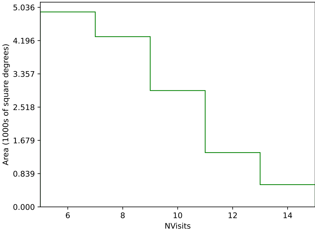
ddf_acor_sf30_lsf40_lsr20_v3.4_10yrs Yr 3-4 g band: NVisits
