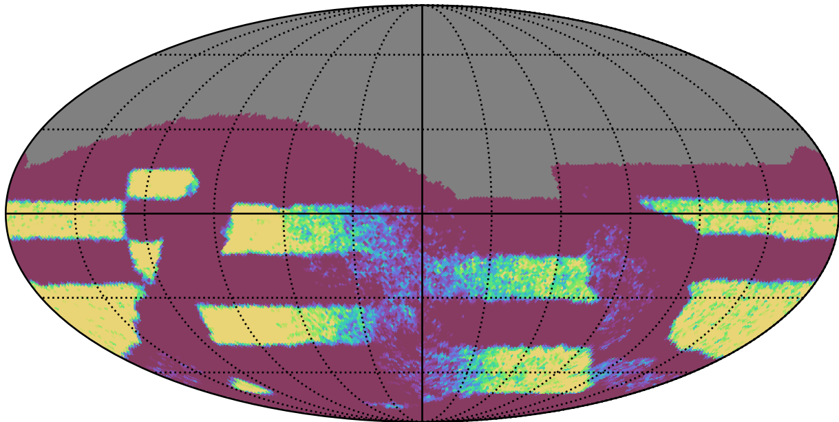
ddf_acor_sf30_lsf40_lsr20_v3.4_10yrs Yr 3-4 all bands: NVisits
