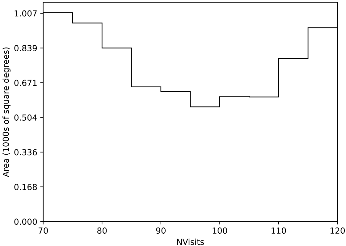
ddf_acor_sf30_lsf40_lsr20_v3.4_10yrs Yr 3-4 all bands: NVisits
