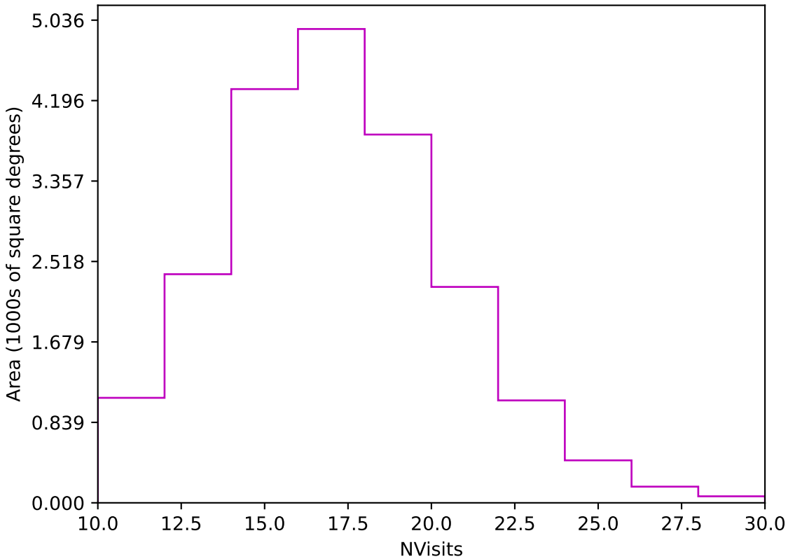
ddf_acor_sf30_lsf40_lsr20_v3.4_10yrs Yr 1 z band: NVisits
