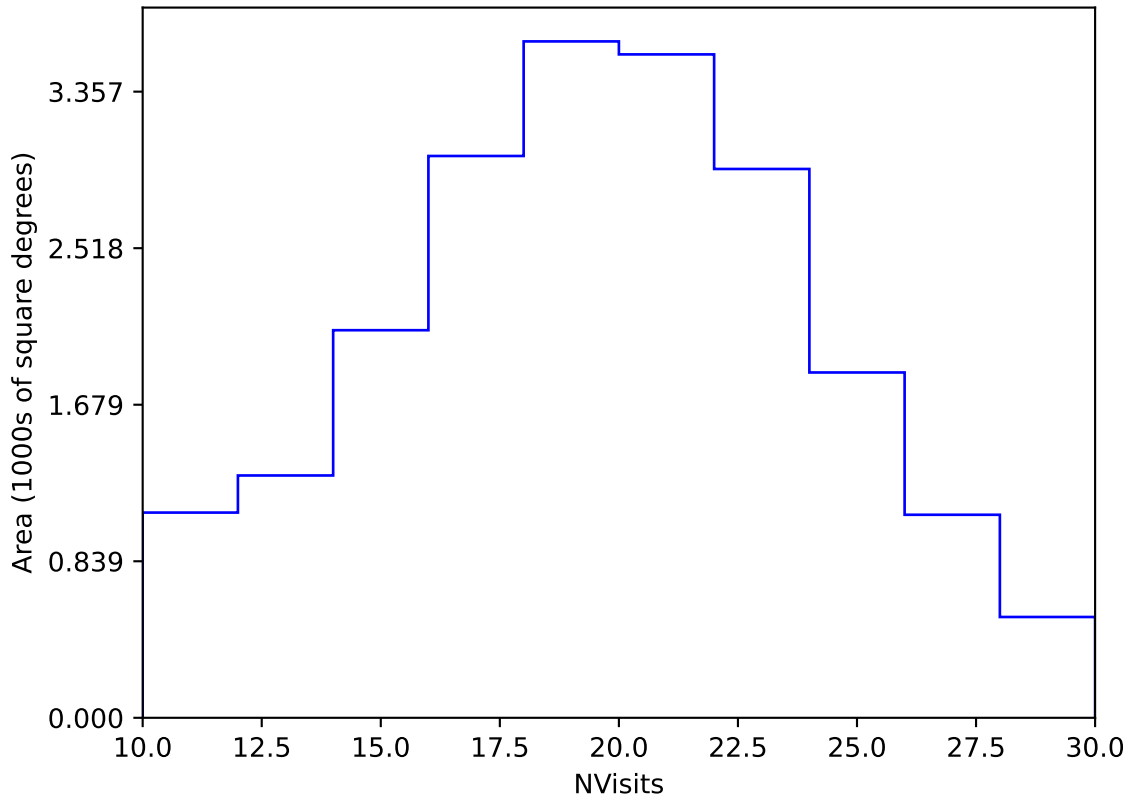
ddf_acor_sf30_lsf40_lsr20_v3.4_10yrs Yr 1 y band: NVisits
