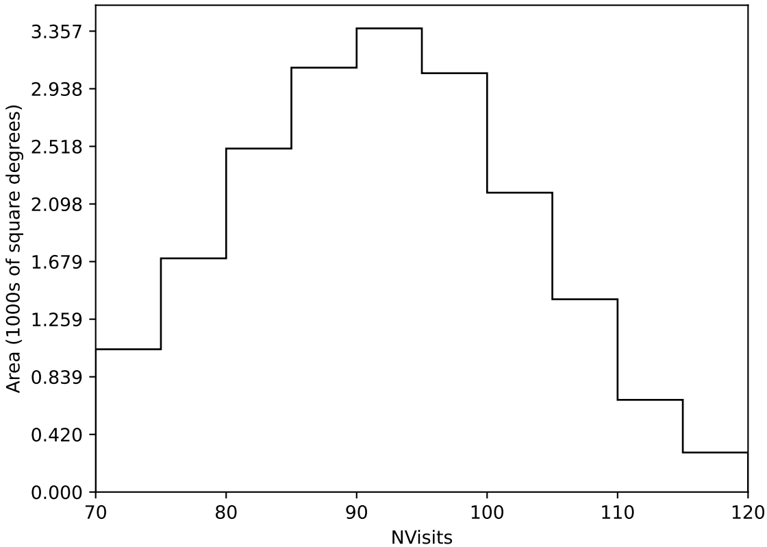
ddf_acor_sf30_lsf40_lsr20_v3.4_10yrs Yr 1 all bands: NVisits
